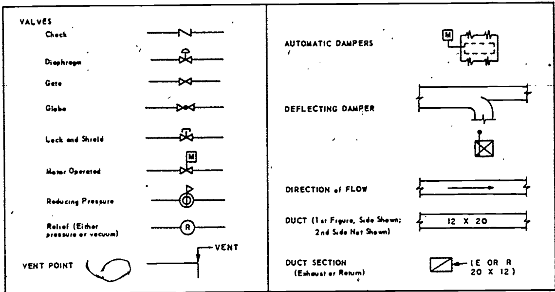
Figure 4-6. Heating symbols.
