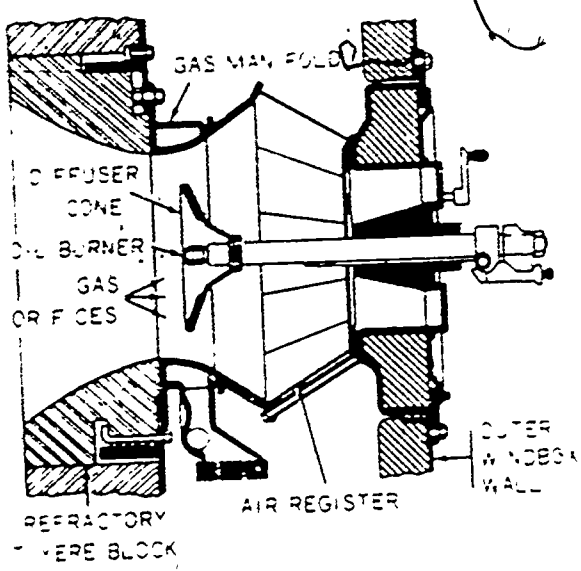
Figure 2-30 A register-type burner with gas orifices at periphery of airstream.
