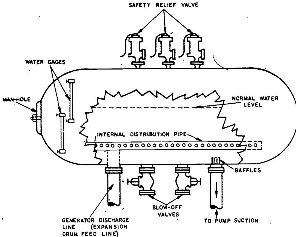
Figure 1-8. Saturated steam cushion expansion drum.
