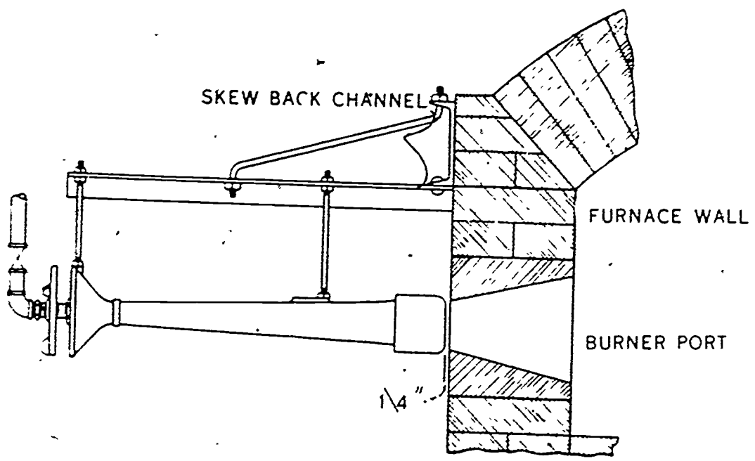
Figure 2-25. An inshot gas burner.
