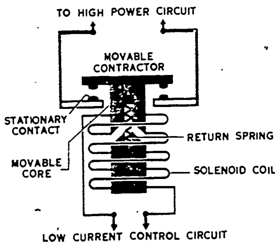
Figure 2-30. Common solenoid.
