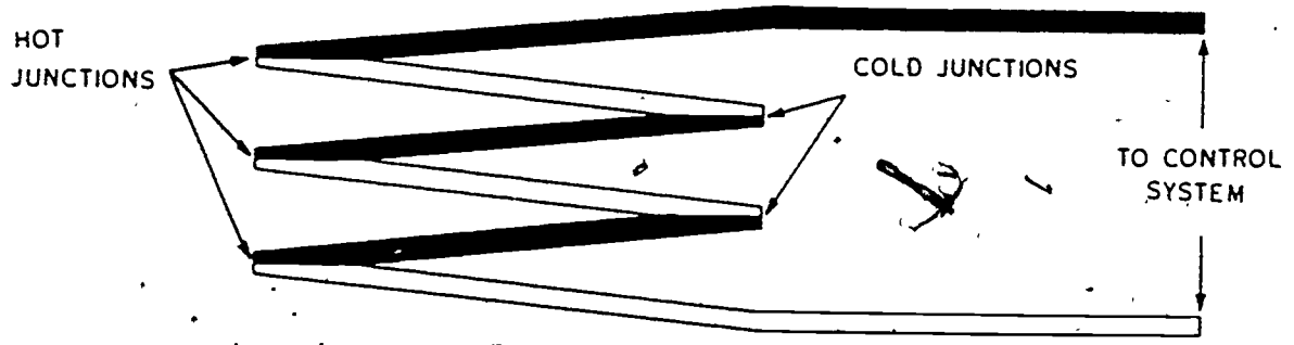
Figure 2-35. A thermopile.
