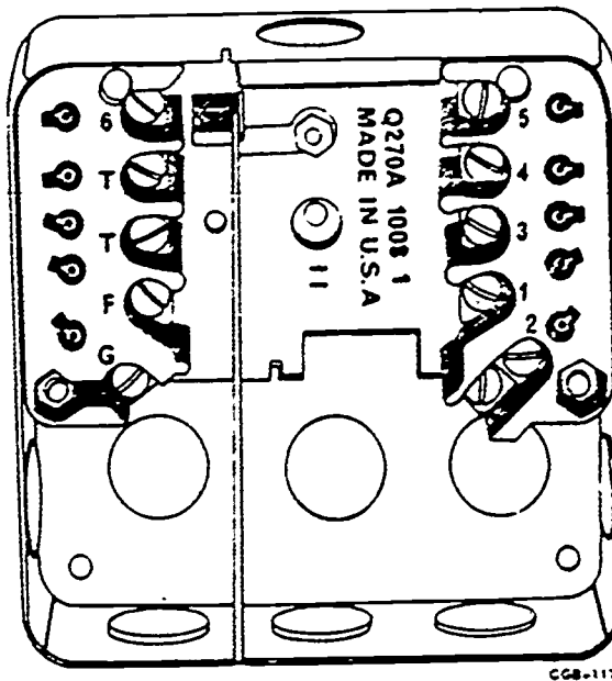
Figure 2-42. Relay subbase.
