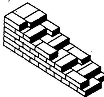
Figure 3-6. A bond for a 1 3/4-inch wall.
