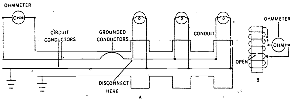
Figure 1-17. Ohmmeter connections
