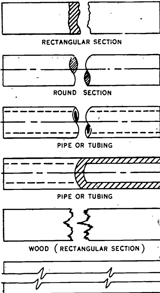
Figure 4-9. Conventional breaks.
