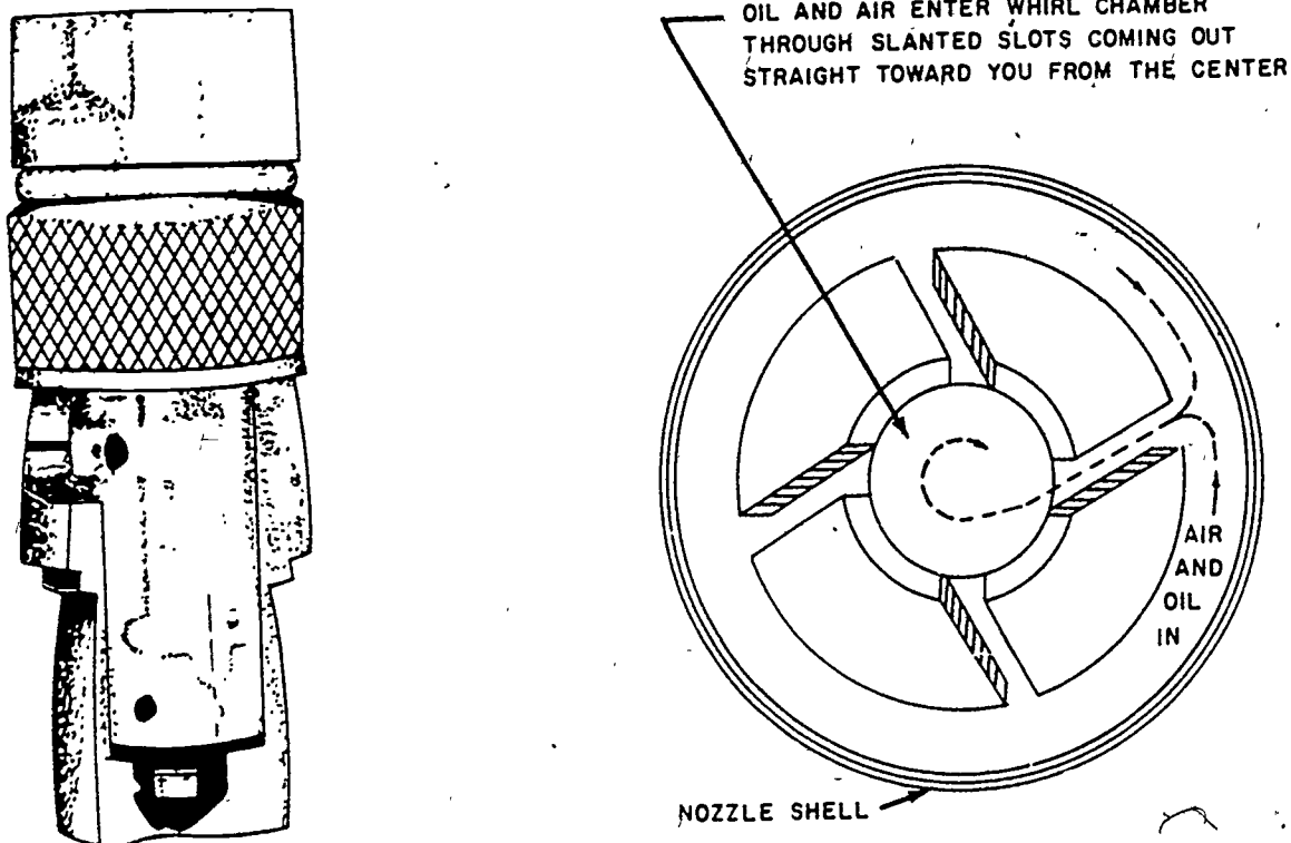
Figure 2-4 Low-pressure nozzle and a cutaway view of the nozzle.
