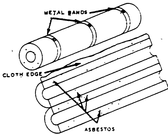
Figure 3-28 Tube insulation.
