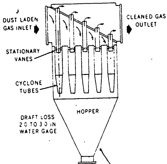
Figure 4-8. Multiple cyclone collector.
