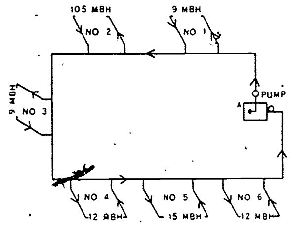
Figure 4-12. One-pipe water circulation system.
