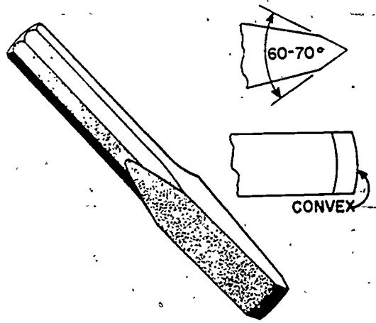
Figure 4-36. Cold chisel.
