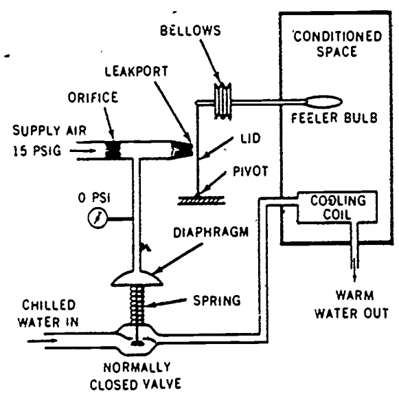
Figure 2-48. Simple bleed control principle.
