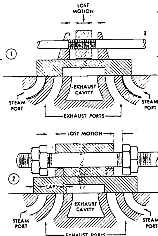
Figure 2-20. Two methods of providing lost motion in a duplex pump slide valve.
