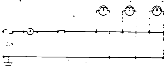
Figure 1-15. Ammeter connections.
