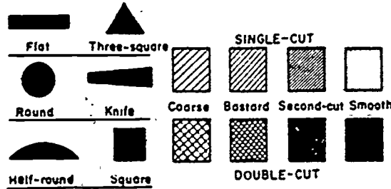
Figure 4-32. File.
