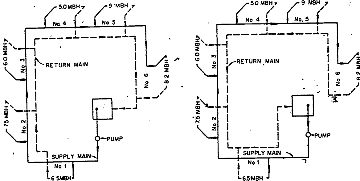
Figure 4-14. Two-pipe systems.
