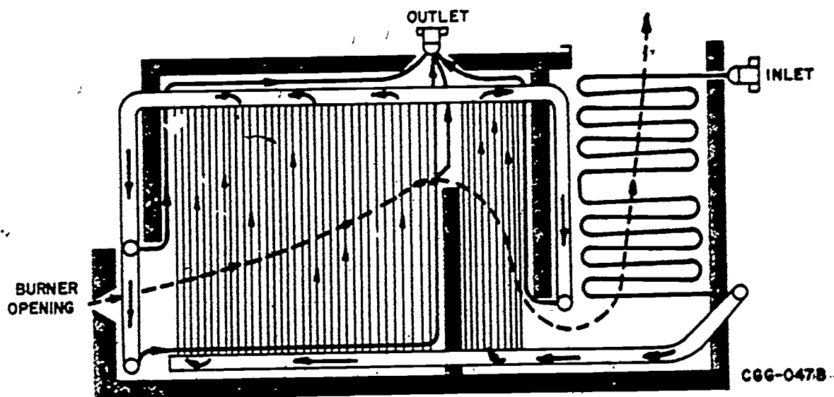
Figure 1-6. Counterflow economizer HTW generator.
