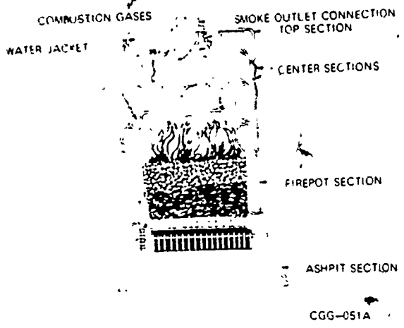
Figure 4-1 A typical round cast iron boiler.
