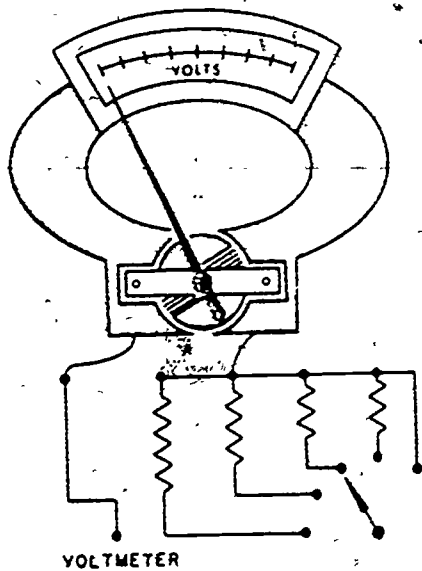
Figure 1-12. Diagram of a multirange voltmeter.
