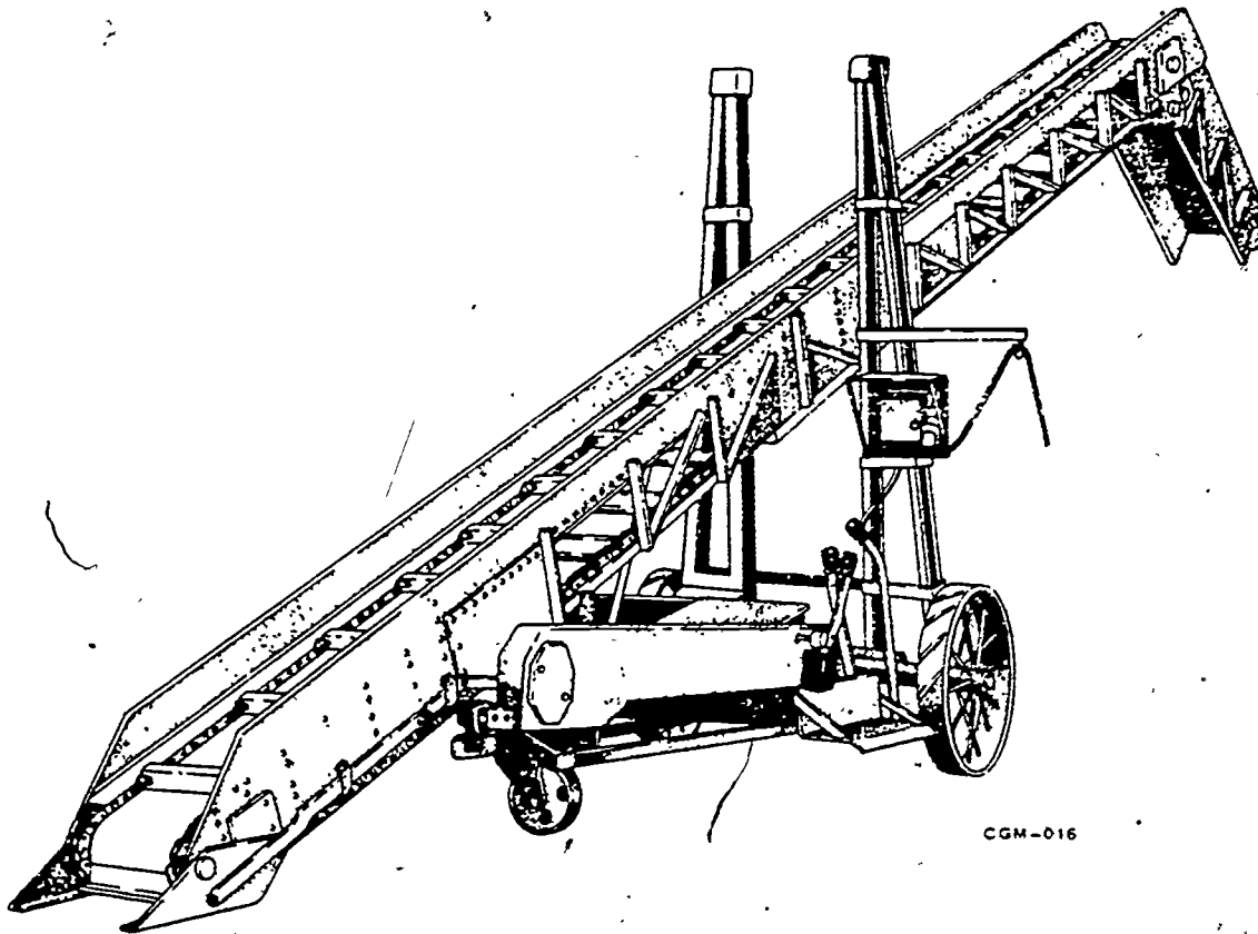
Figure 5-6. Conveyer stacker.
