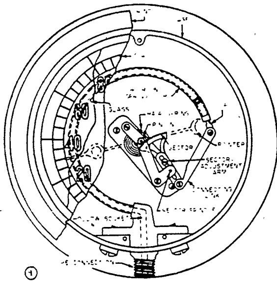
Figure 2-21. A typical Bourdon spring pressure gauge.
