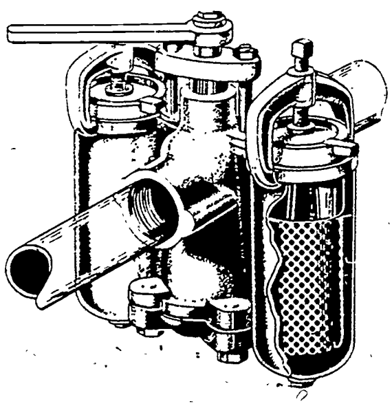
Figure 5-9. A typical duplex fuel oil strainer.
