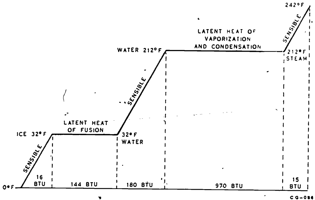
Figure 4-2. Sensible and latent heat.
