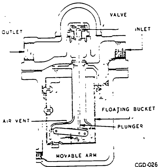
Figure 3-19. Bucket trap with trap closed.
