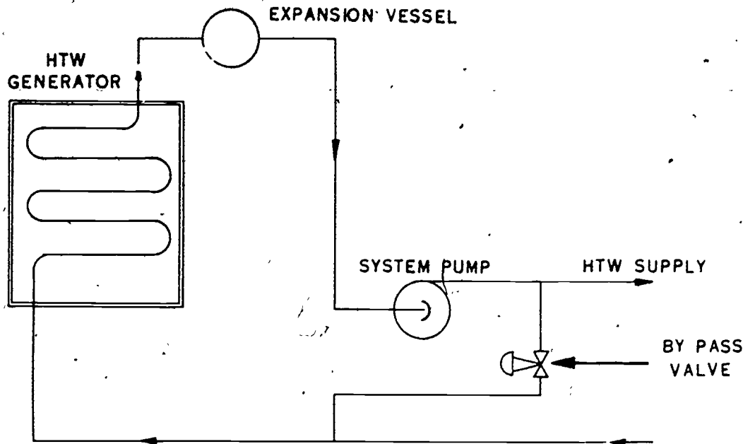
Figure 1-14. Bypass valve.
