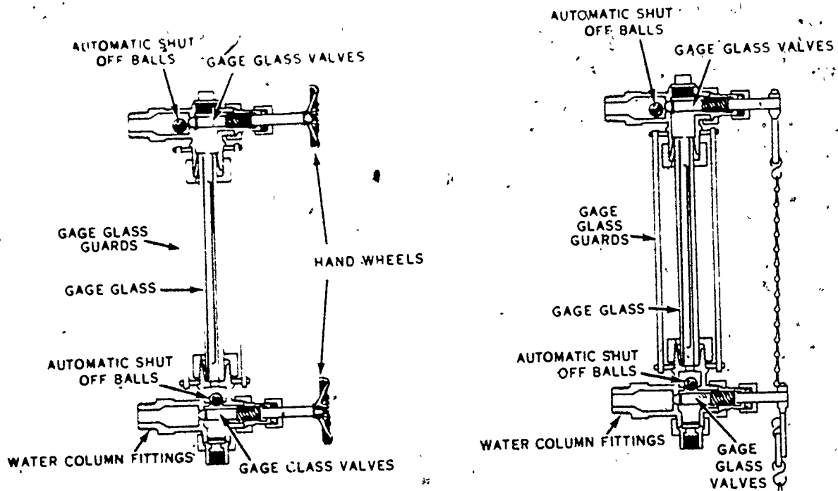
Figure 2-9. Gage glasses.
