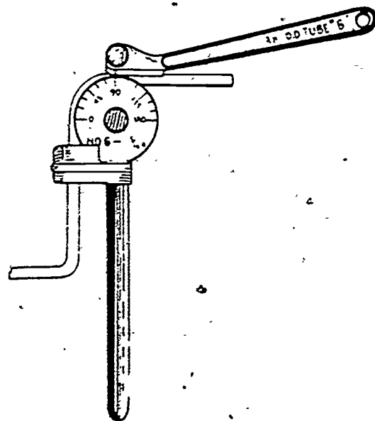
Figure 4-52. Tube bender.
