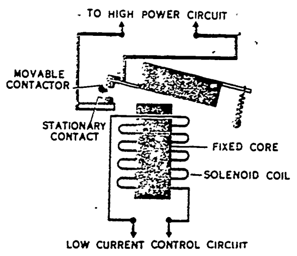
Figure 2-29. Common relay
