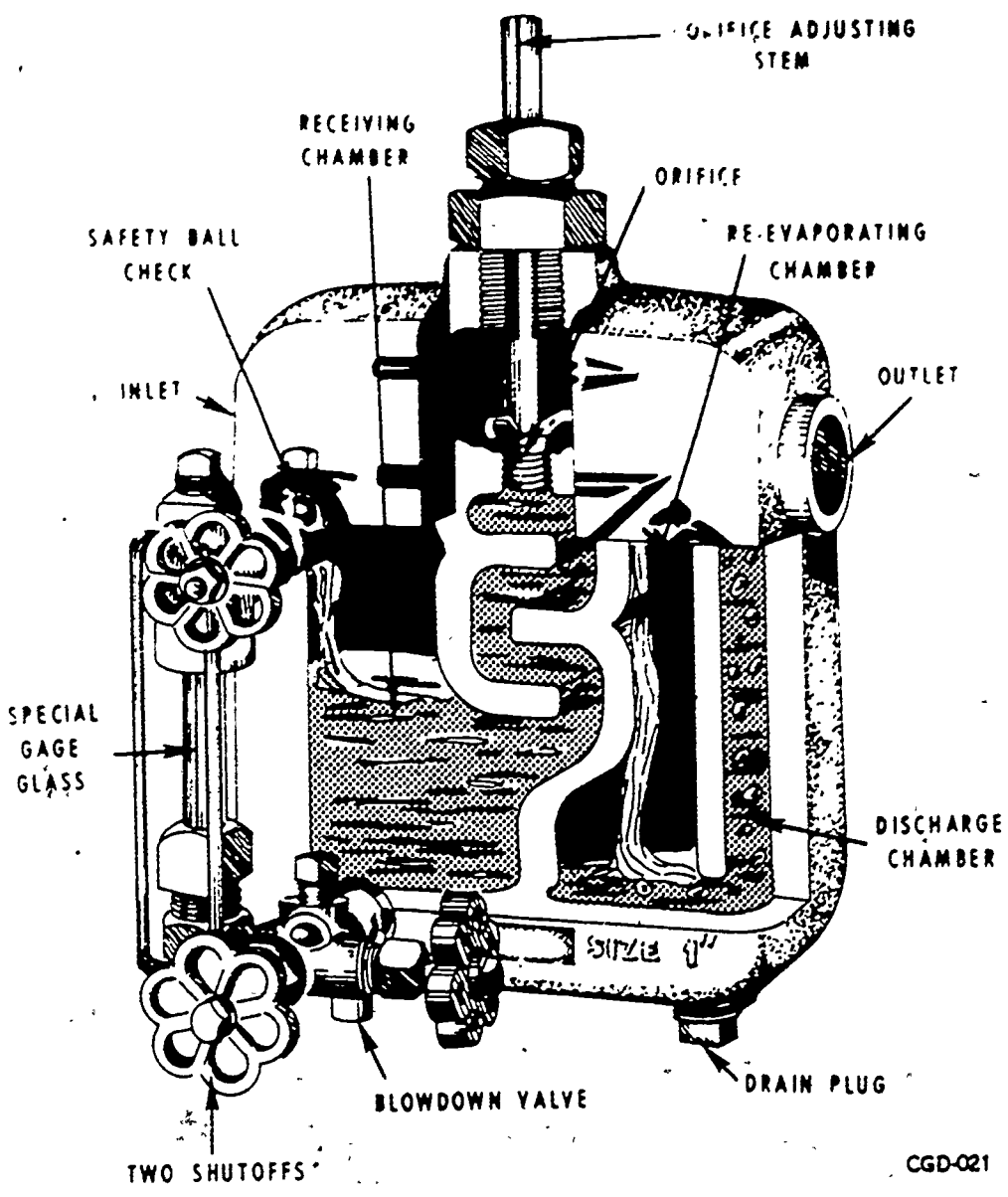
Figure 3-24. Throttling trap.
