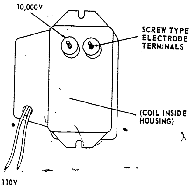
Figure 2-15. An ignition transformer.
