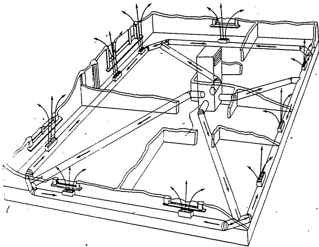
Figure 3-5 Perimeter loop.
