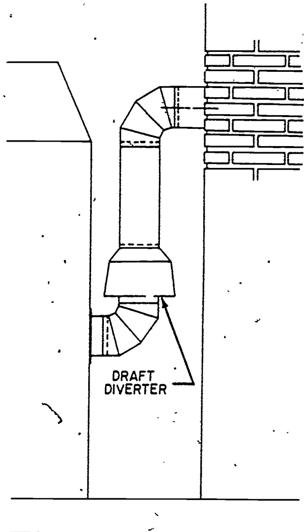
Figure 1-8. A typical draft diverter.
