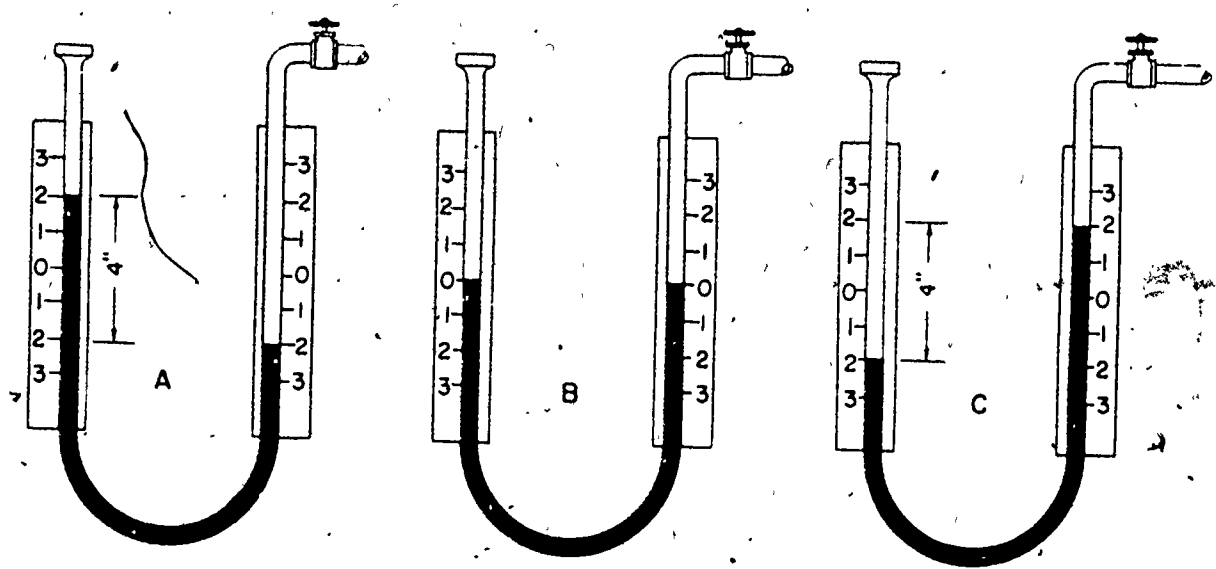
Figure 2-22. Open manometers having different readings.
