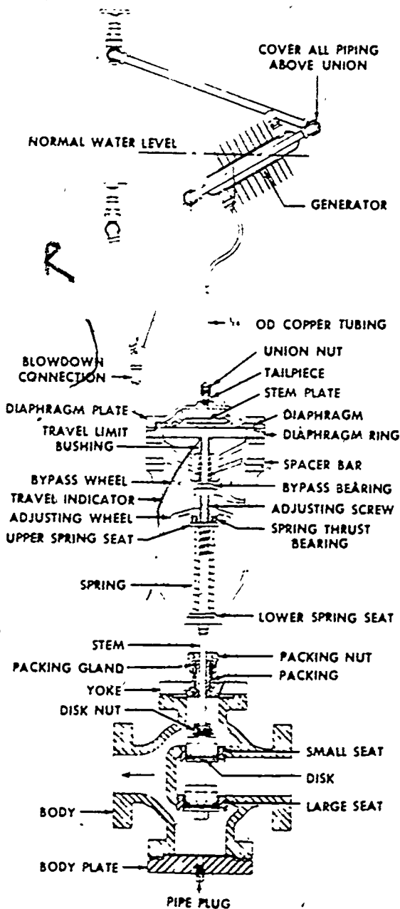
Figure 2-17. A vapor generator feedwater regulator.
