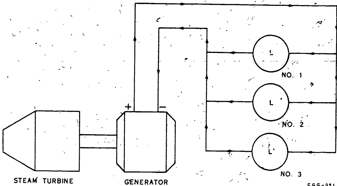
Figure 1-5. Parallel circuit.
