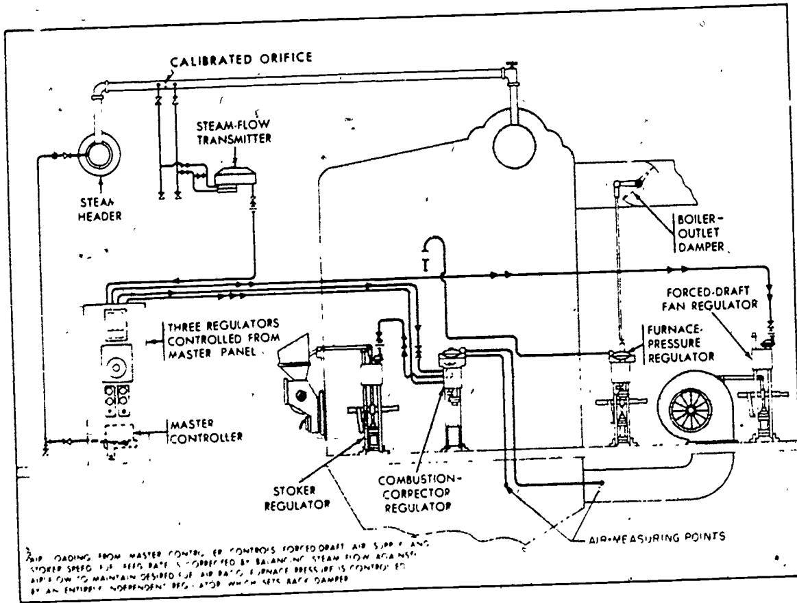
Figure 2-25. Metering-type combustion control for large boiler: direct airflow measurement.
