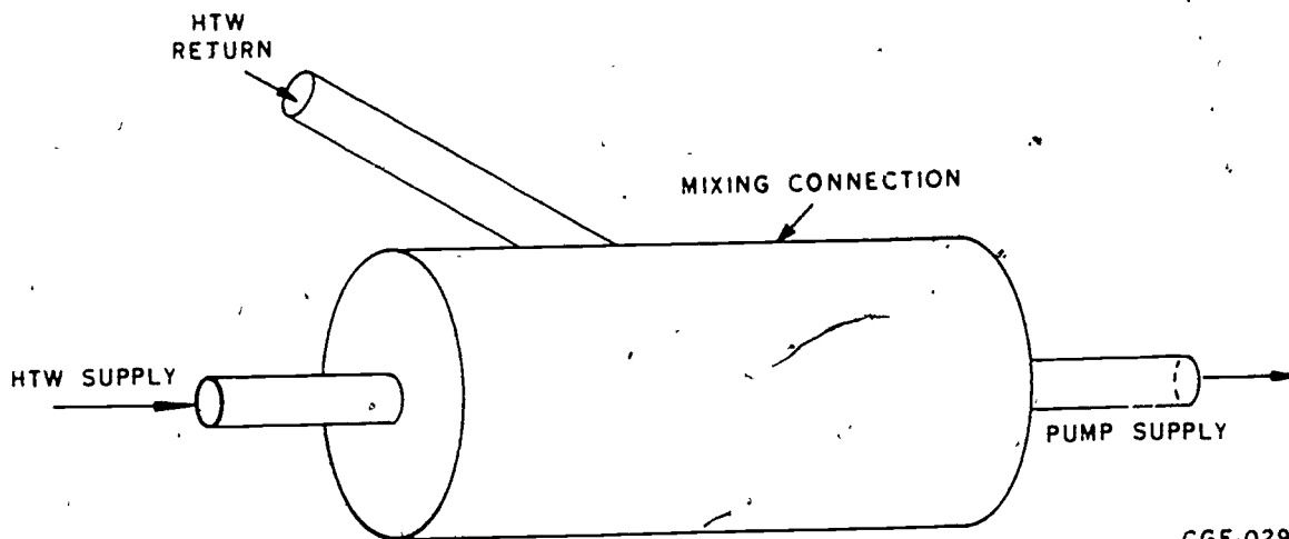
Figure 1-16. Mixing connection.
