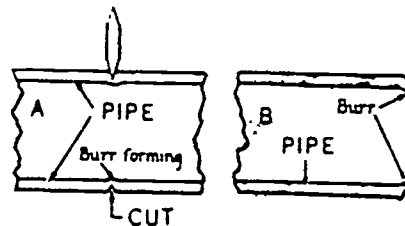
Figure 3-13. The results of cutting pipe with a pipe cutter.
