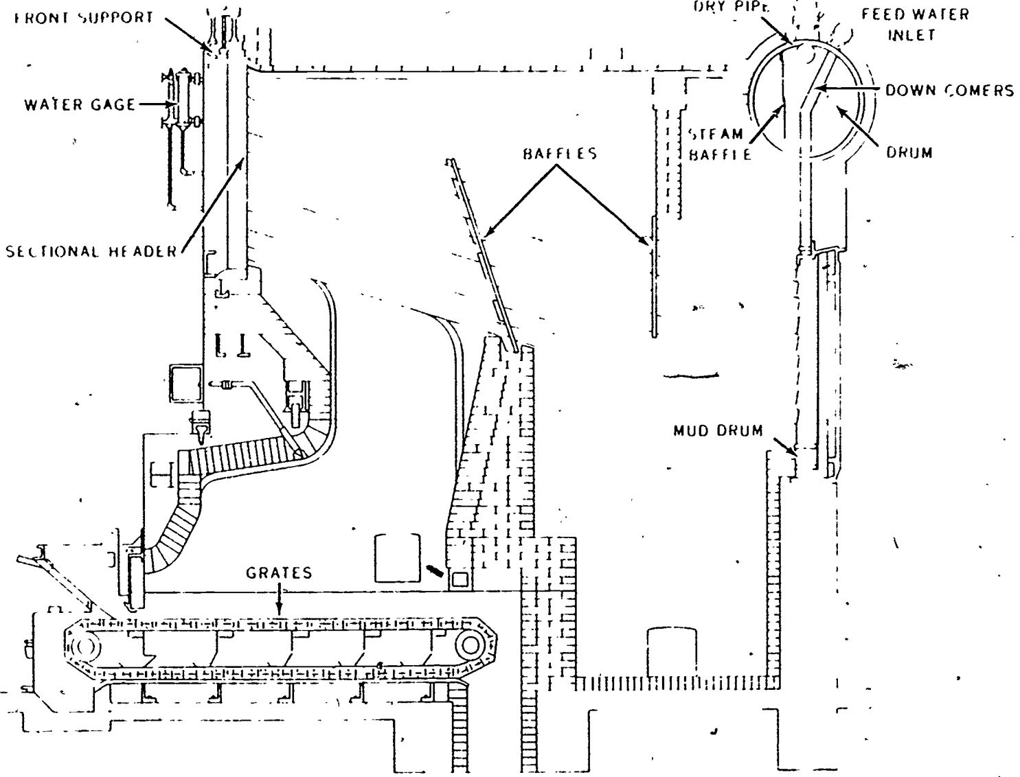
Figure 2-5. A sectional-header cross-drum boiler.
