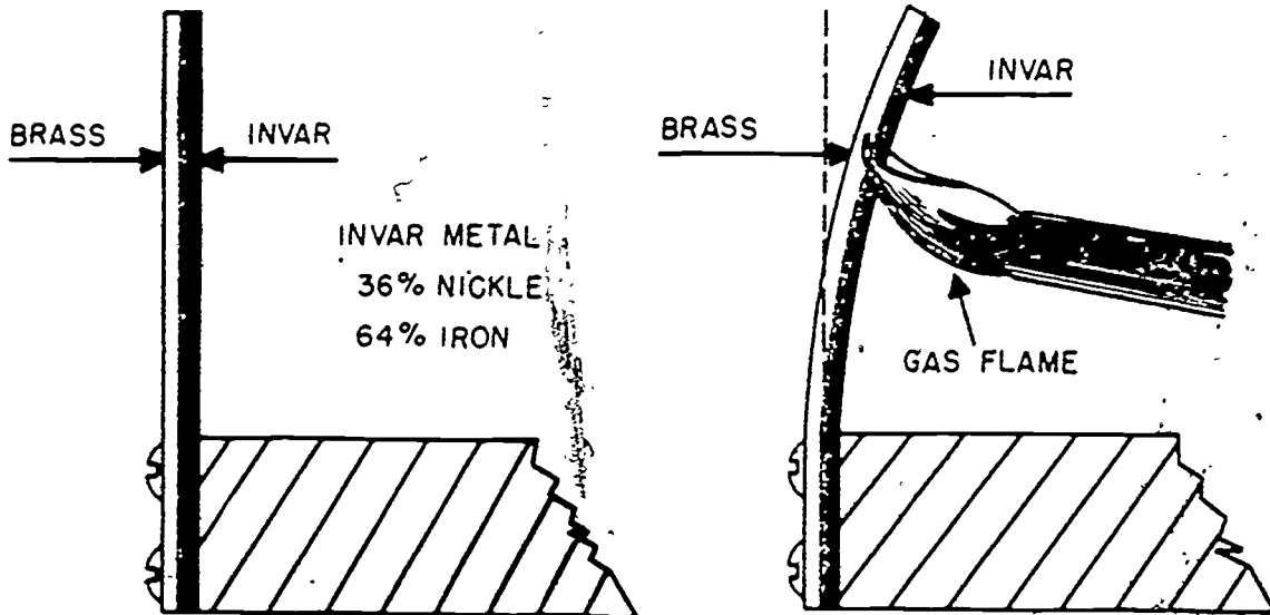
Figure 2-6. Bending of bimetallic strip.
