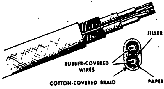
Figure 2-14. Nonmetallic type cable.
