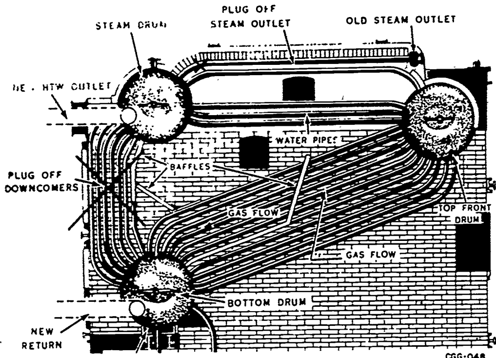
Figure 1-1. Converted steam boiler.
