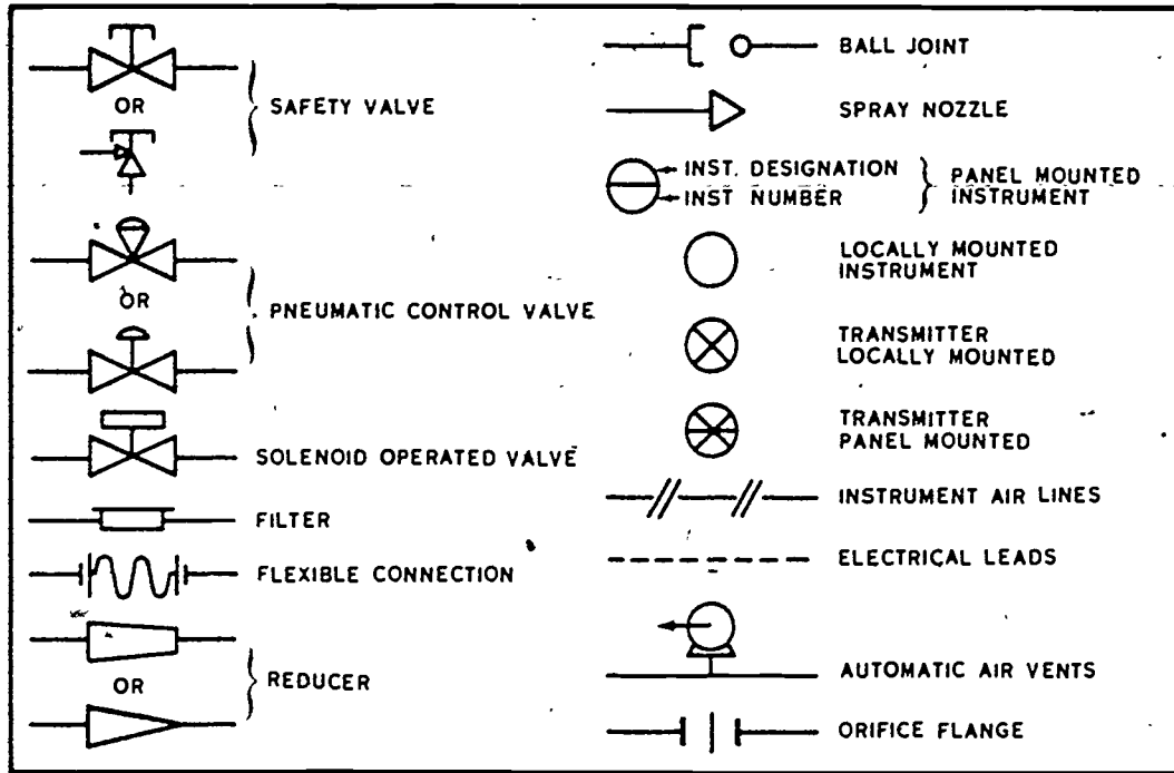
Figure 4-4. Piping symbols.
