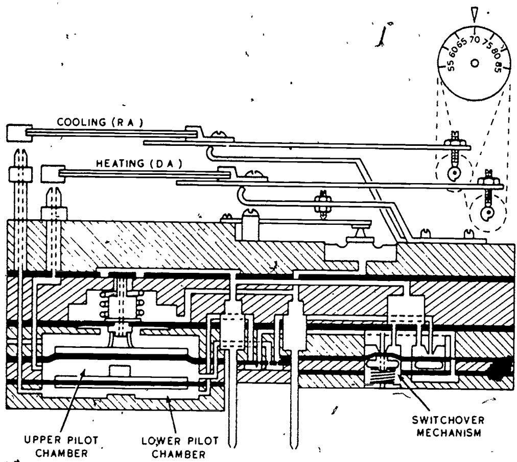
Figure 2-54. Heating-cooling thermostat.
