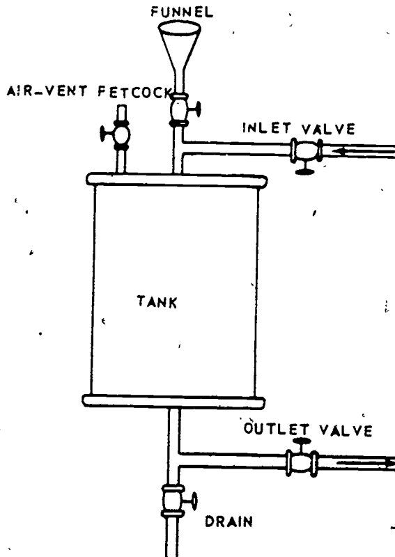
Figure 5-14. Closed feeder.
