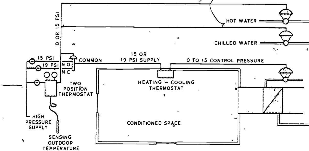
Figure 2-53. Application of a heating-cooling thermostat.
