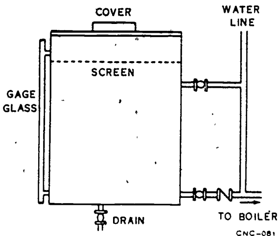
Figure 5-15. Open feeder.
