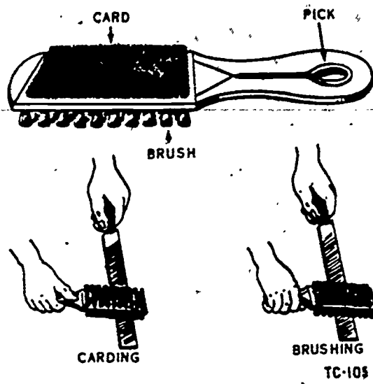
Figure 4-35. File card.
