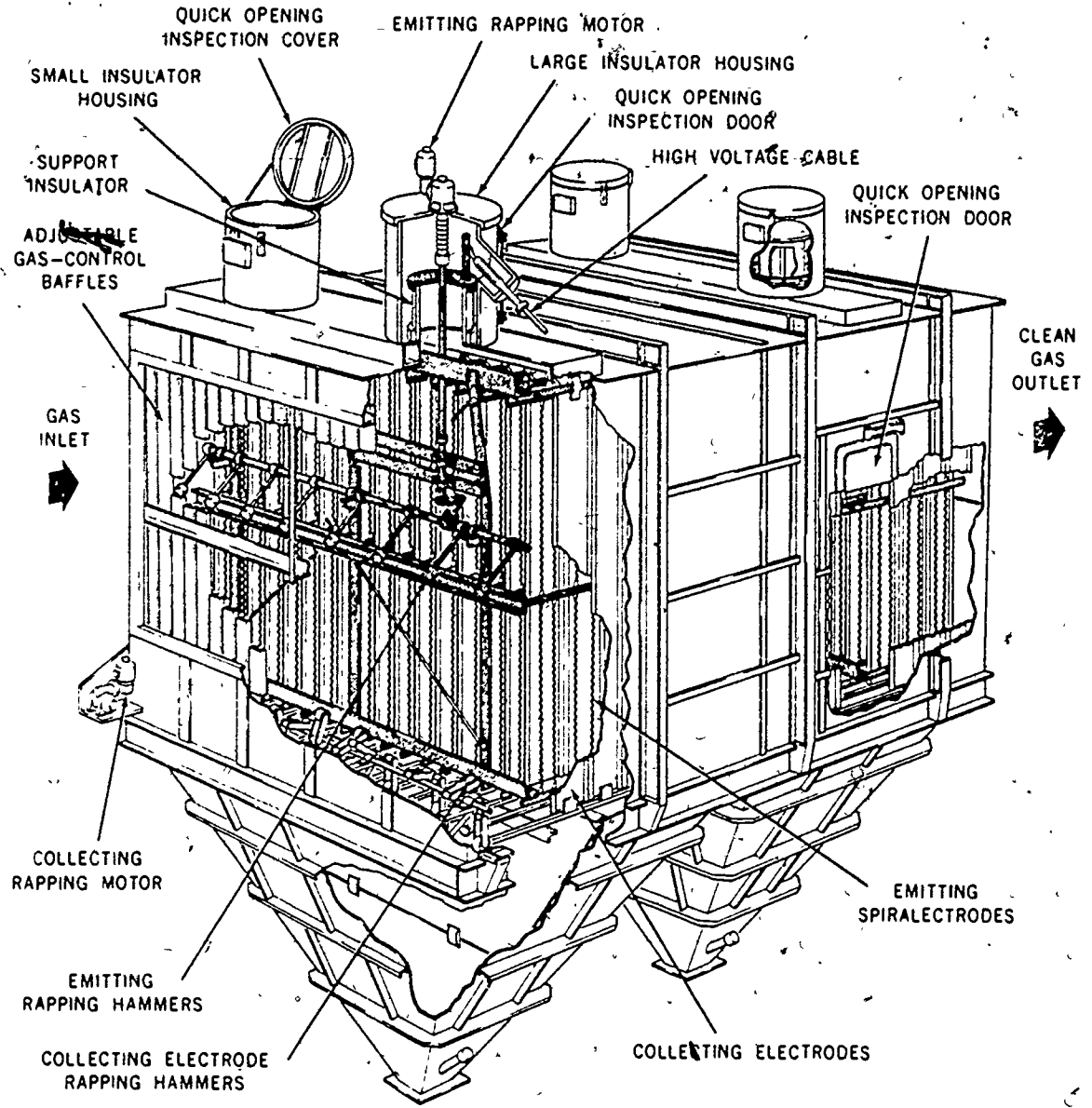
Figure 4-9. Electrostatic precipitator.
