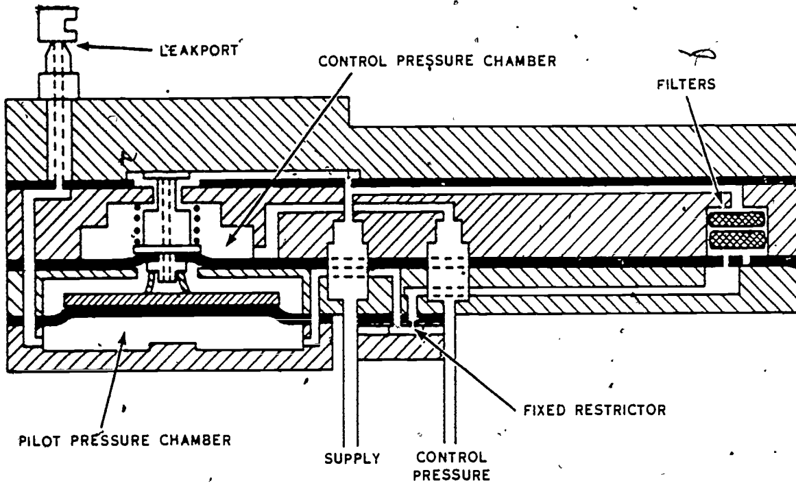
Figure 2-50. Pilot operated pneumatic relay.
