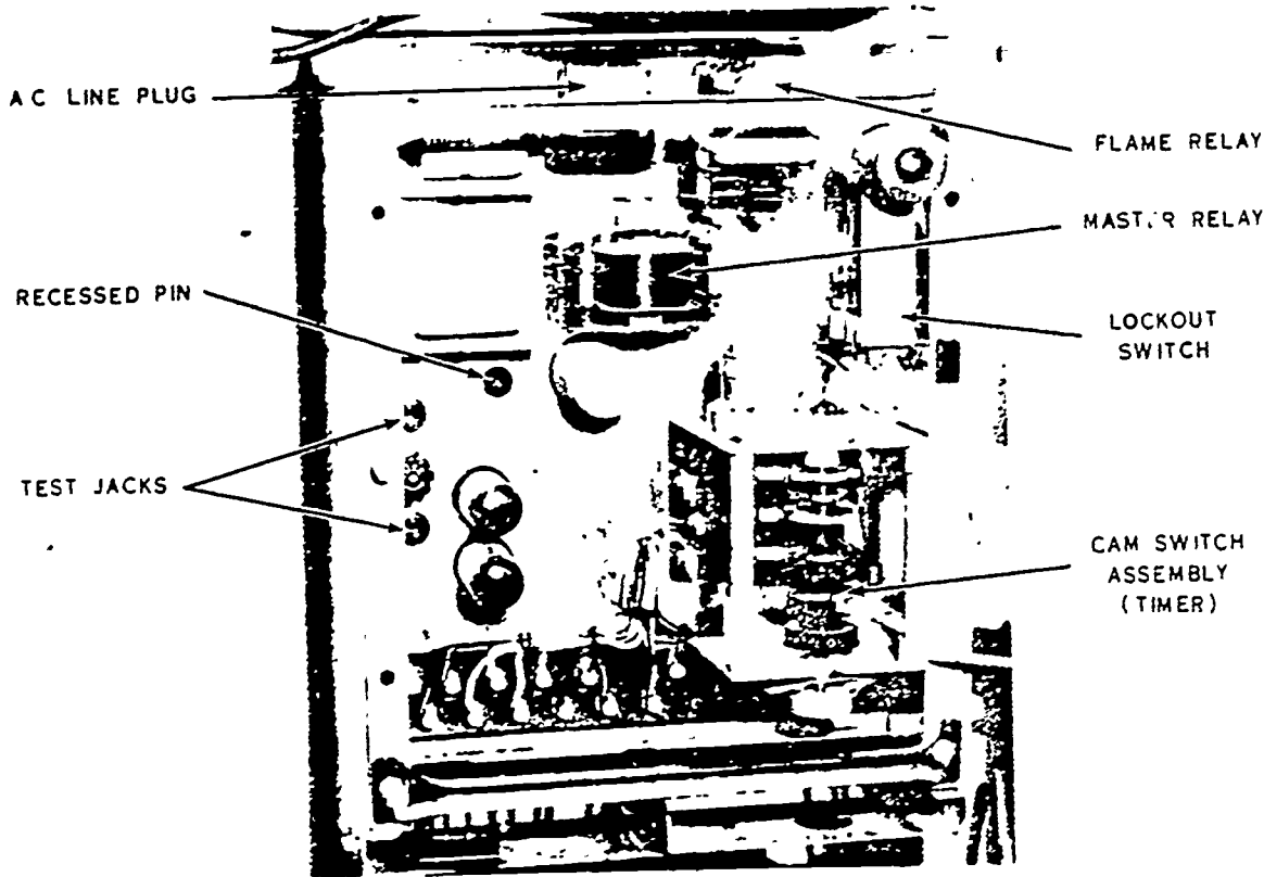
Figure 2-46. Programing control.
