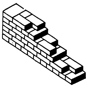
Figure 3-5. A bond for a 9-inch wall.
