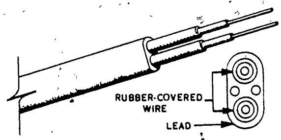
Figure 2-15. Lead-sheathed duplex cable.
