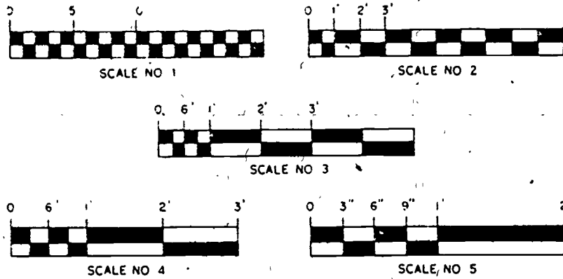
Figure 4-13. Graphic scales.
