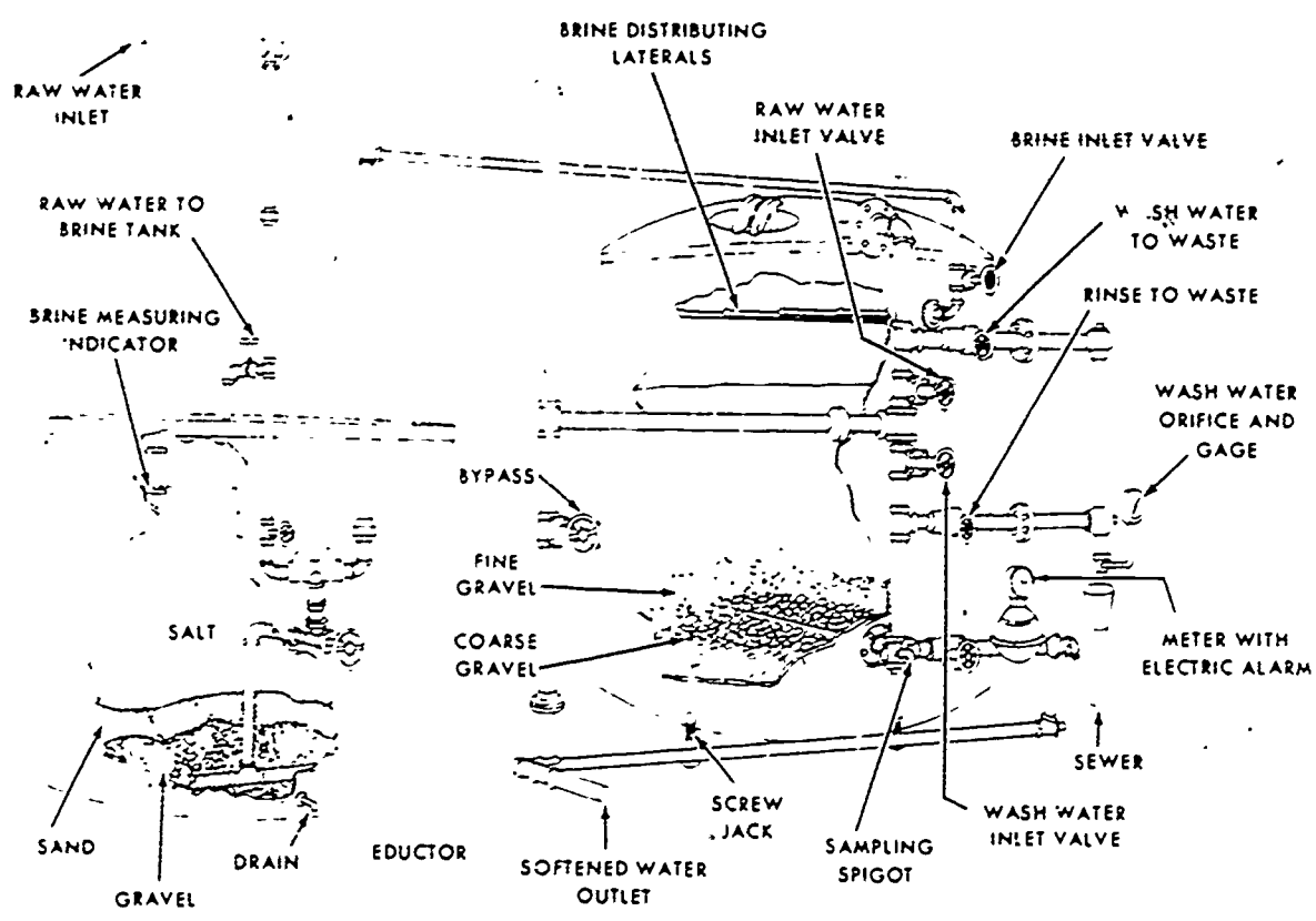
Figure 4-5. Sodium-zeolite softener.
