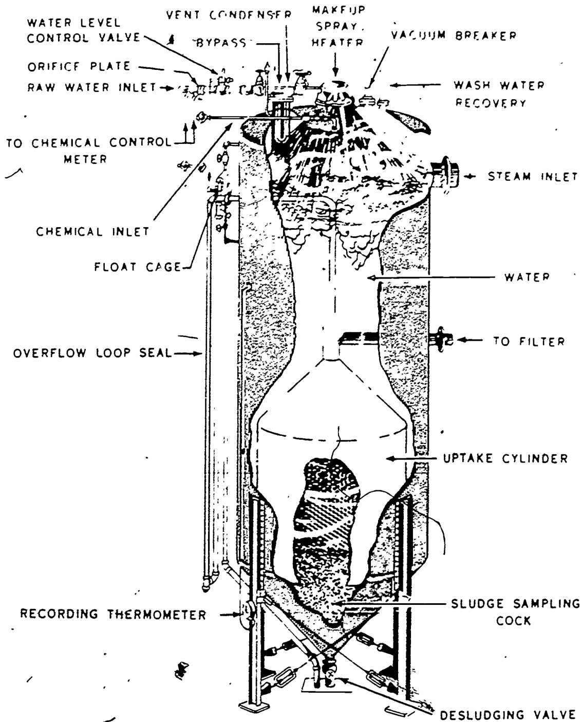
Figure 4-6. Lime-soda softener.
