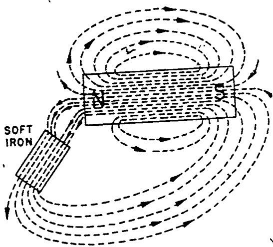
Figure 2-23. Distortion of a magnetic field.
