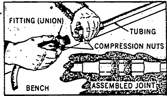
Figure 3-26. Assembly of a flared joint.
