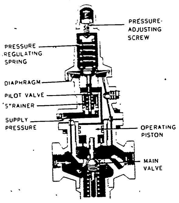
Figure 2-31. A gas pressure regulator.
