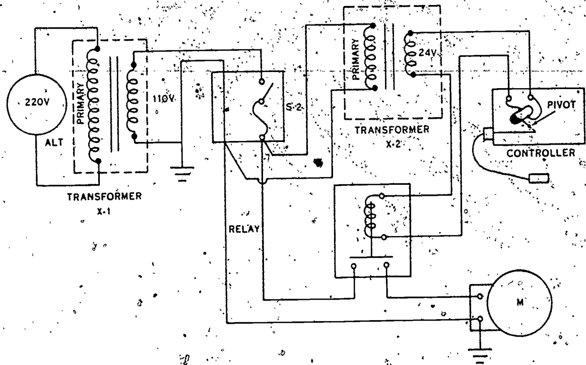
Figure 2-3. Control relay.
