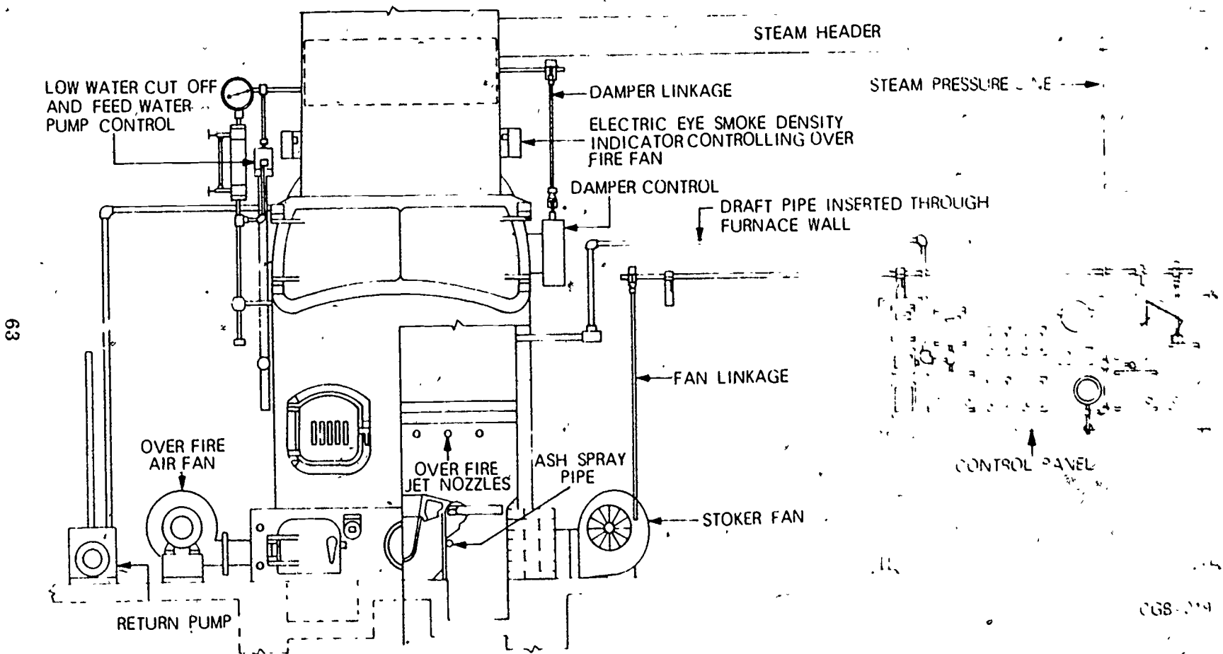
Figure 2-24. Pressure control system for industrial boiler, including smoke control.
