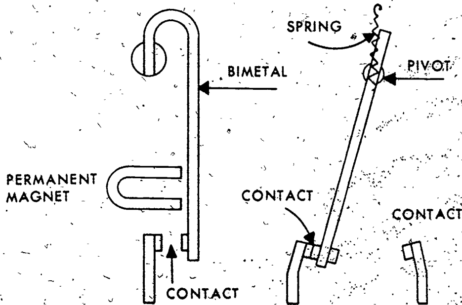
Figure 2-1. Snap-action type switch.
