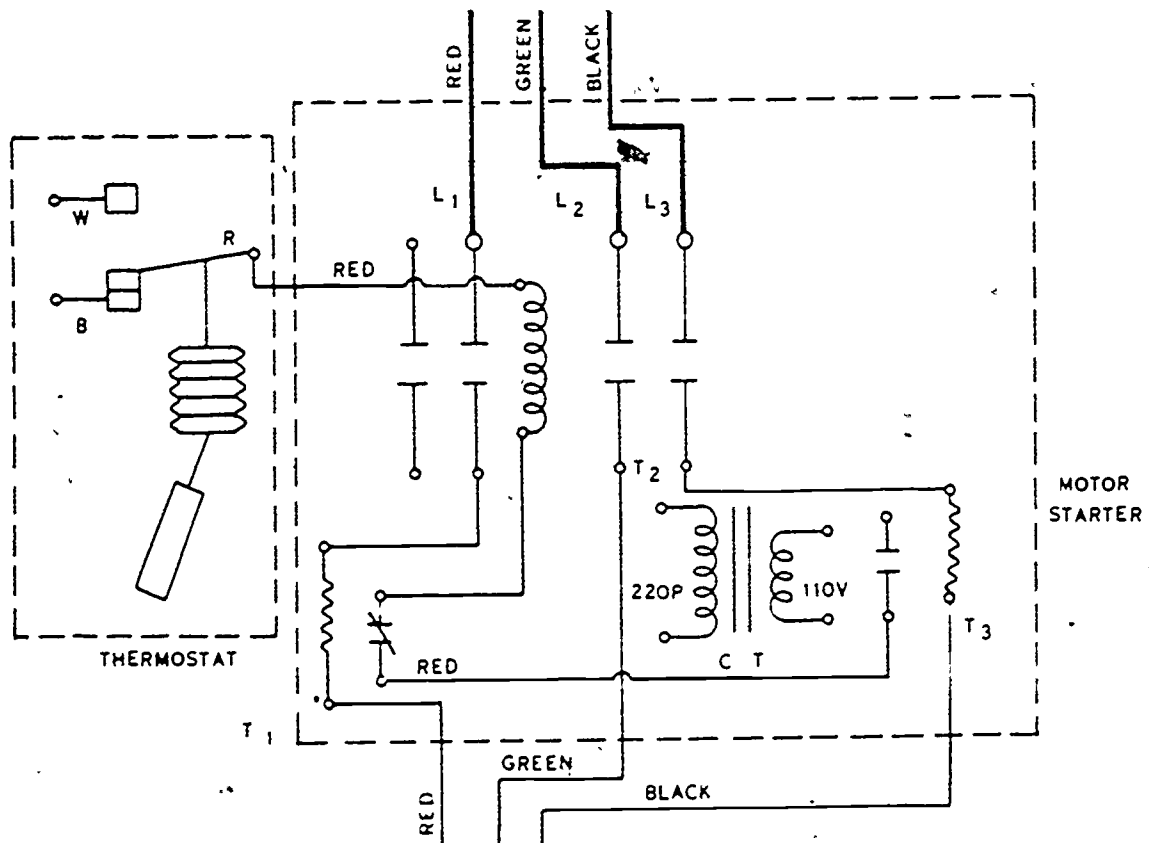
Figure 2-4. Magnetic starter.
