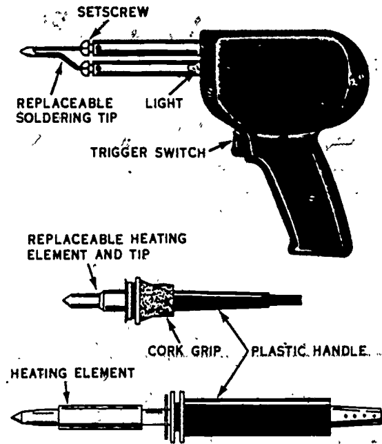
Figure 4-46. Soldering guns.
