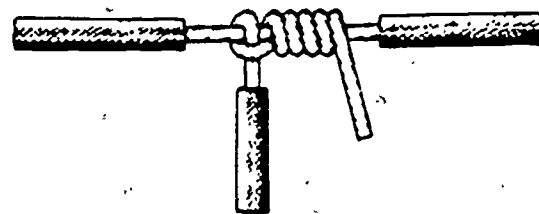
Figure 2-19. A tap splice.
