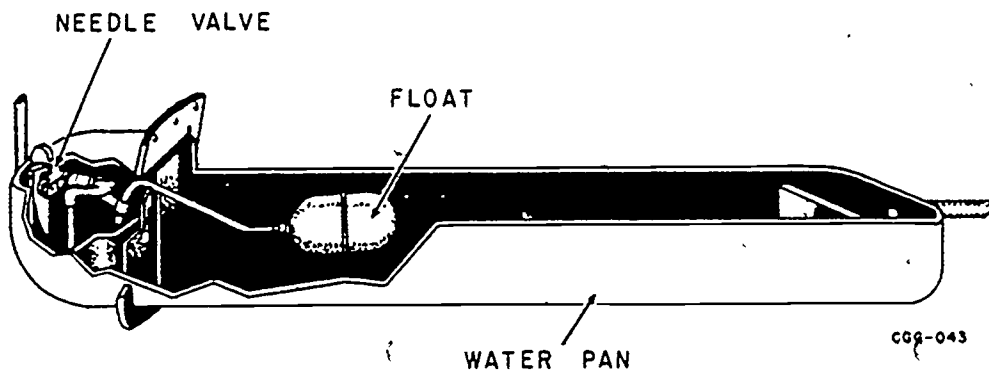
Figure 3-19. A typical humidifier.
