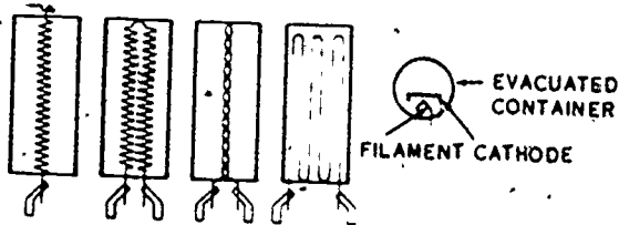
Figure 2-34. Indirect heated cathodes.
