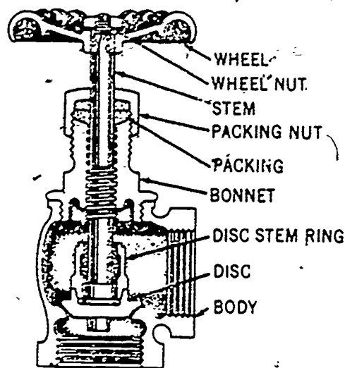
Figure 3-8. Cross section of an angle valve.
