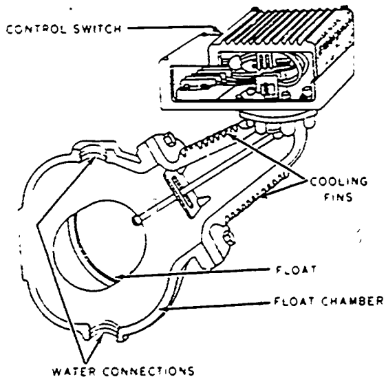
Figure 2-19 A typical boiler feedwater controller
