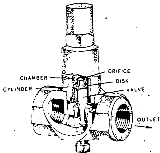
Figure 3-23. Impulse trap.
