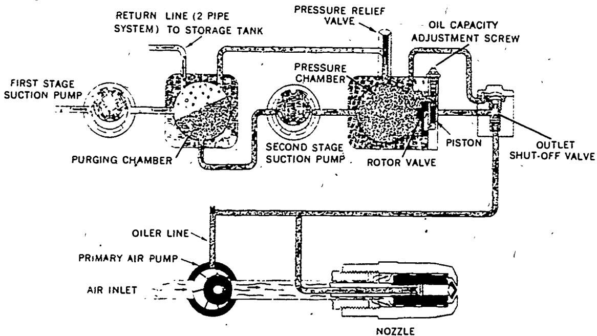
Figure 2-20. Flow diagram of two-stage low-pressure air atomizing burner system.
