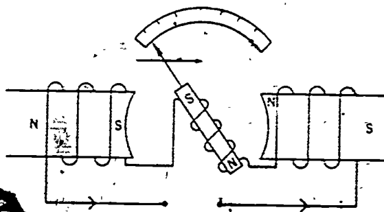
Figure 1-11. Simple diagram of a dynamometer movement.
