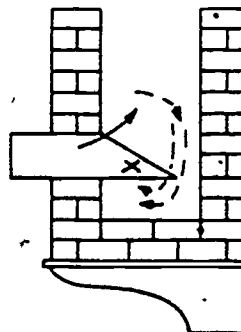
Figure 1-19. Toothpick joint.
