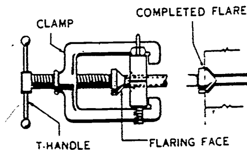
Figure 3-25. Positioning the clamp and making the flare.
