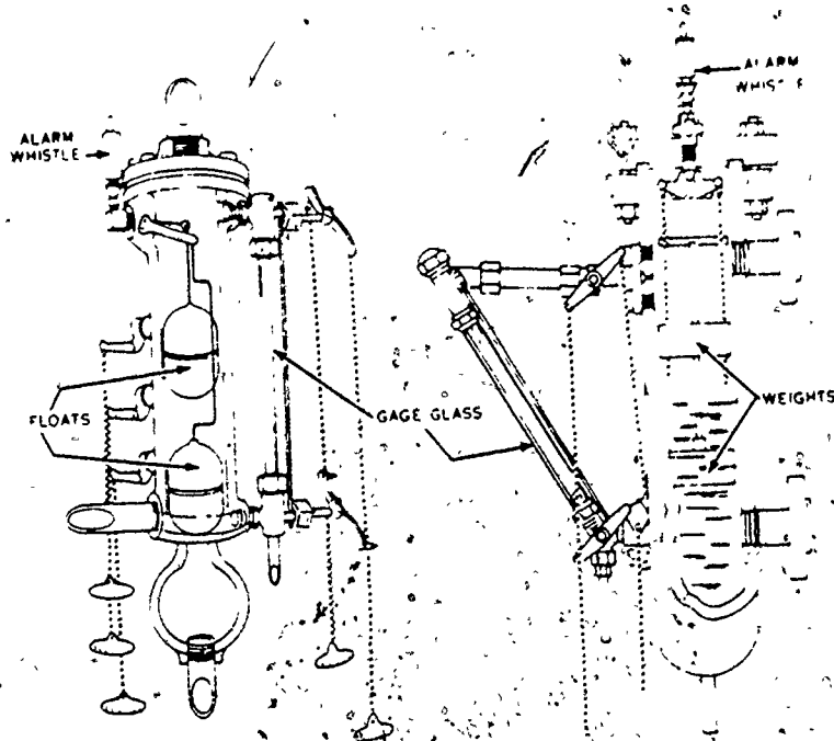
Figure 2-10. Water columns.
