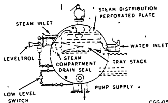
Figure 1-4. End cutaway of a direct contact heater.
